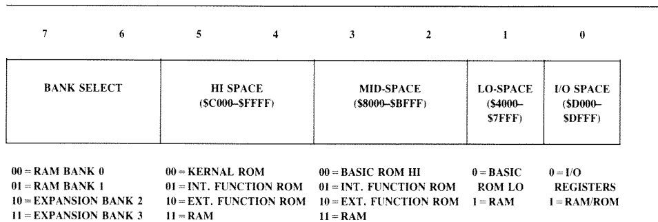
Figure 13-5. Configuration Register
