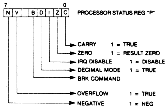
Figure 5-2. 8502 Status Register
